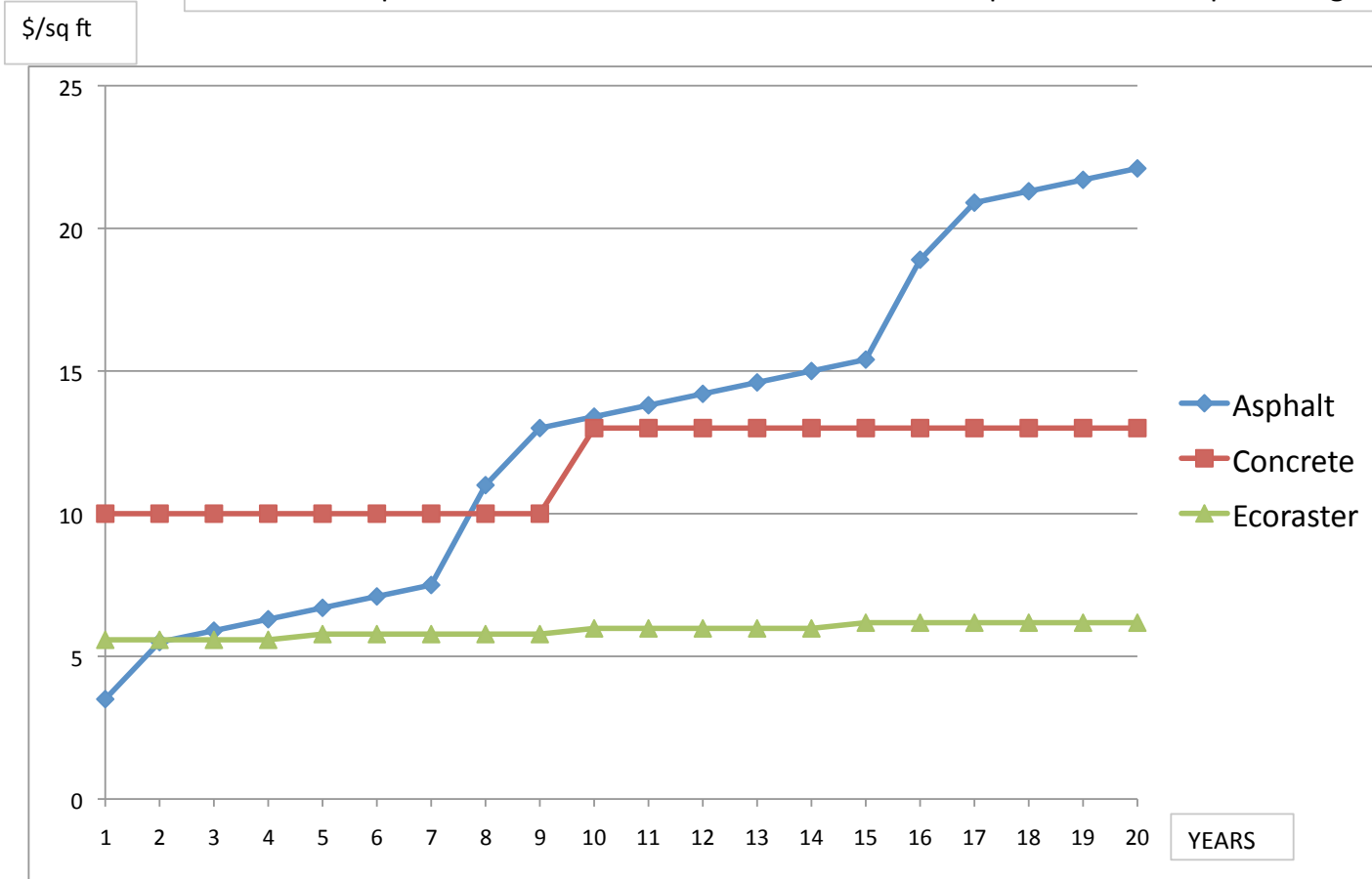
Asphalt, Concrete and ECORASTER® Pavers Graphic of Cost $/sq ft through 20 years
